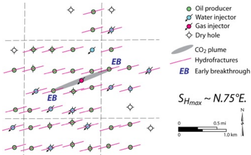
Figure 2.2.2. Wells in the vicinity of the CO 2 injection pilot test (the injector, Well B-19-10 #2 is indicated by the red-filled circle near the center), showing the likely orientation of hydraulic fractures in the direction of maximum horizontal compressive stress, ~ North 75° East, the preferential migration of the CO 2 plume in the direction of the fractures, and the location of wells where early breakthrough of CO 2 was observed.
