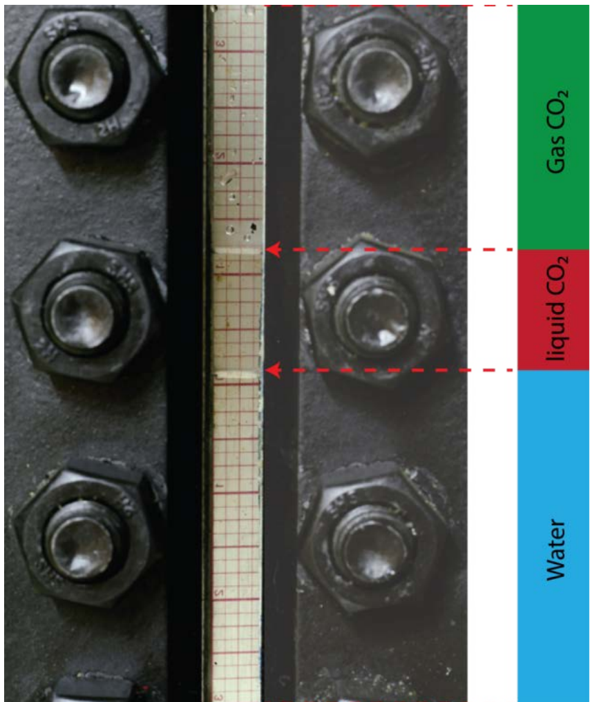
Figure 2.3.2. High-pressure, high-temperature cell for study of CO 2 -oil phase behavior. The gaseous CO 2 /liquid CO 2 and the liquid CO 2 /water phase boundaries are visible (upper and lower arrows, respectively).
