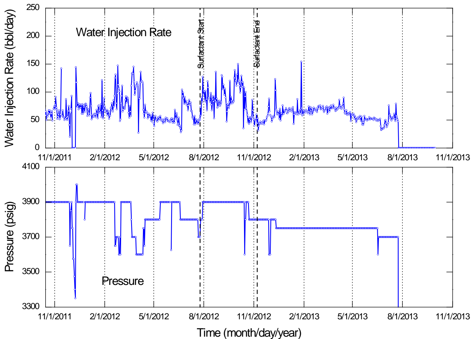
Figure 2.6.8. Rates (top) and pressures (bottom) of water injection into Well B-19-10 #2 in the inverted five-spot test pattern at Citronelle, from October 15, 2011, to September 30, 2013. Surfactant treatment began on July 25, 2012 and ended on November 7, 2012. The well was shut in for repair of a tubing leak on July 25, 2013.
