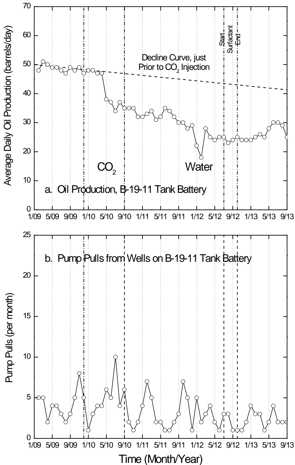
Figure 2.6.4. Response to CO 2 injection at Tank Battery B-19-11. a. Oil production at B-19-11 Tank Battery, which receives fluids from Well B-19-11, from February 2009 to September 2013. b. Number of times per month that power oil pumps in wells on B-19-11 Tank Battery had to be pulled for maintenance or replacement, from February 2009 to September 2013.
