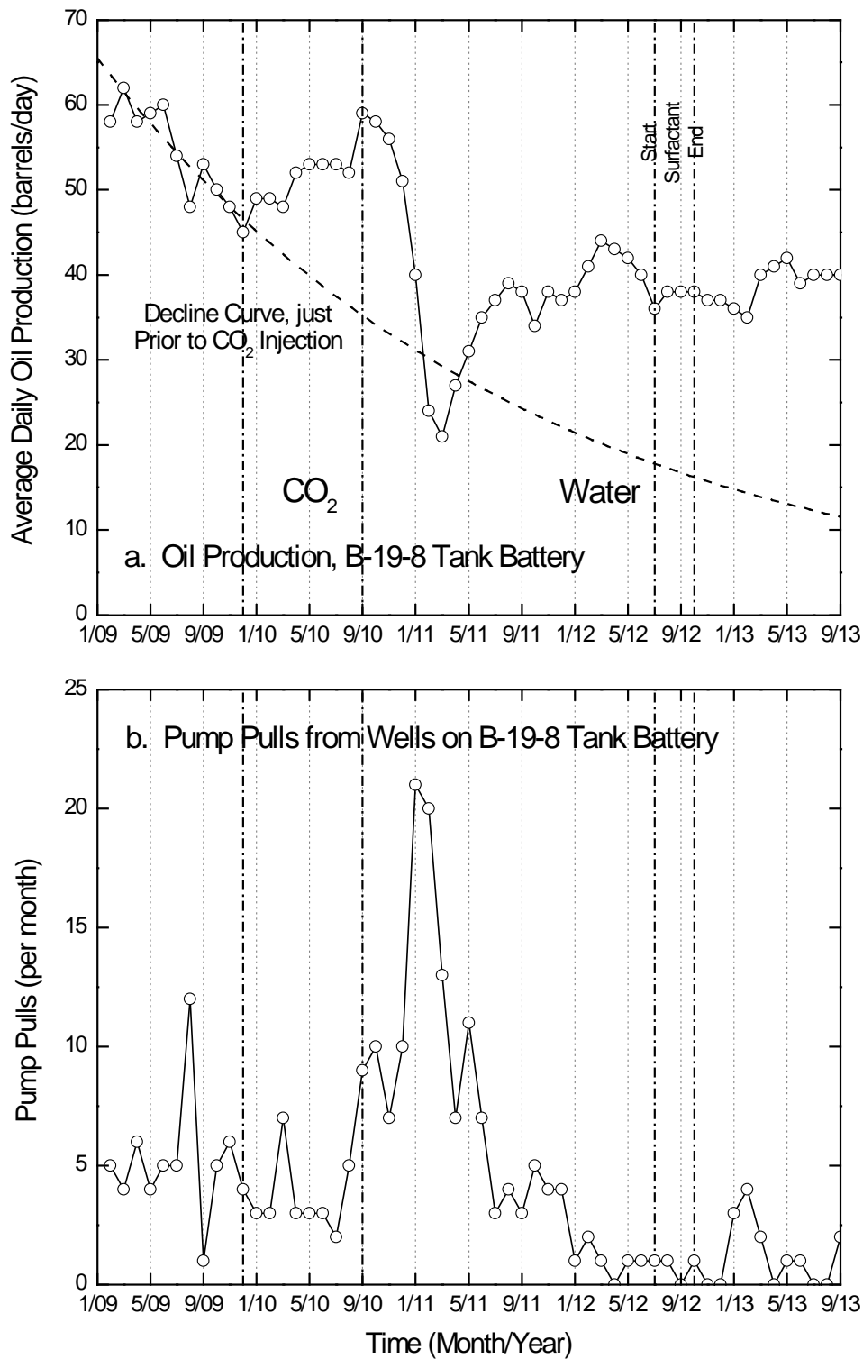
Figure 2.6.3. Response to CO 2 injection at Tank Battery B-19-8. a. Oil production at B-19-8 Tank Battery, which receives fluids from Wells B-19-7, B-19-8, and B-19-9, from February 2009 to September 2013. b. Number of times per month that power oil pumps in wells on B-19-8 Tank Battery had to be pulled for maintenance or replacement, from February 2009 to September 2013.
