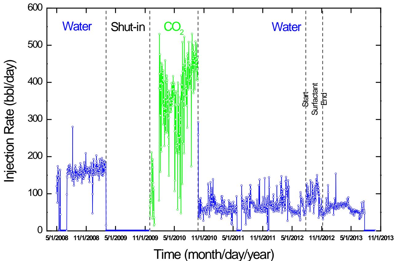
Figure 2.6.7. History of the rates of water and CO 2 injection into Well B-19-10 #2, by volume, from May 2, 2008, to September 30, 2013. We are trying to determine the causes of the loss in injectivity on returning to water injection following the CO 2 slug.
